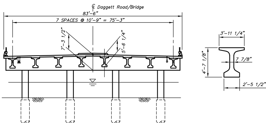
Eight lines of spliced bulb-tee girders were used. Illustration: DMJM Harris.
